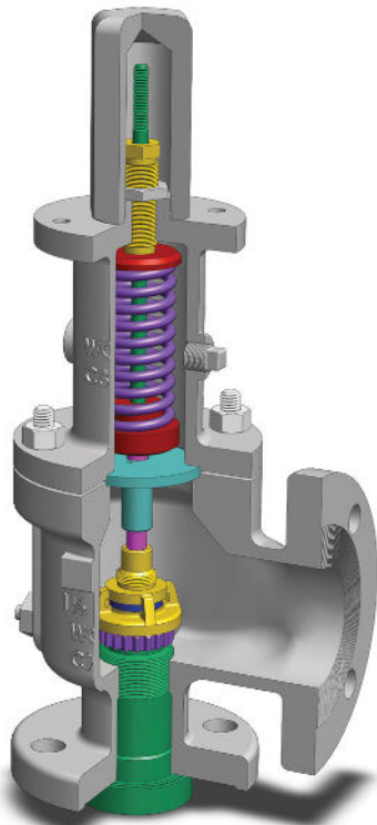
R Series Pressure Relief Valve
