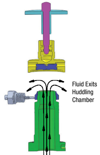
Valve Opens, Force PA_h Acting on Disc
