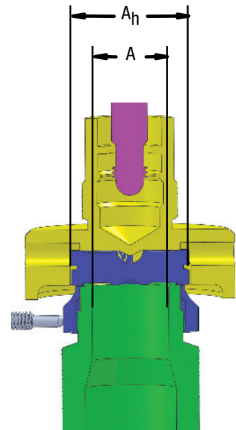
Relationship of Nozzle Area to Huddling Chamber Area
